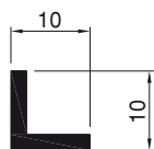
Art.Nr. A8110 L - Winkelprofil 10x10x2
